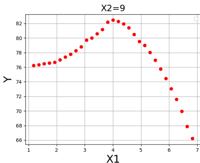
Fig. 13 Response trend for Catalyst loading.
