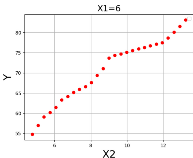
Fig. 14 Response trend for Methanol:oil molar ratio.
