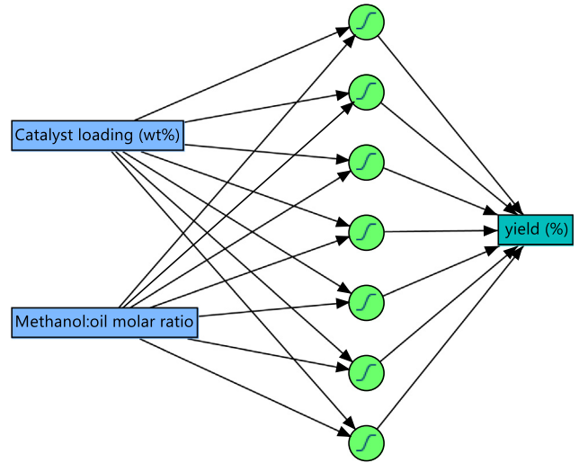
Fig. 1 Prediction of biodiesel production by ANN model.
