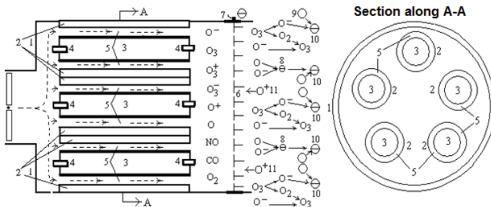
Figure 2. The formation of the ion-ozone mixture, nitrogen oxides and carbon from the air in the ion-ozonator generator: 1 – the body of the ion-ozonator; 2 – metal electrodes of the ozone generator; 3 – glass electrodes; 4 – contacts of glass electrodes of an ozone generator; 5 – discharge gap; 6 – generator of oxygen ions; 7 – contact of the ion generator; 8 – stable molecular ion; 9 – a neutral atom; 10 – heavy molecular ion; 11 – a positive ion.
