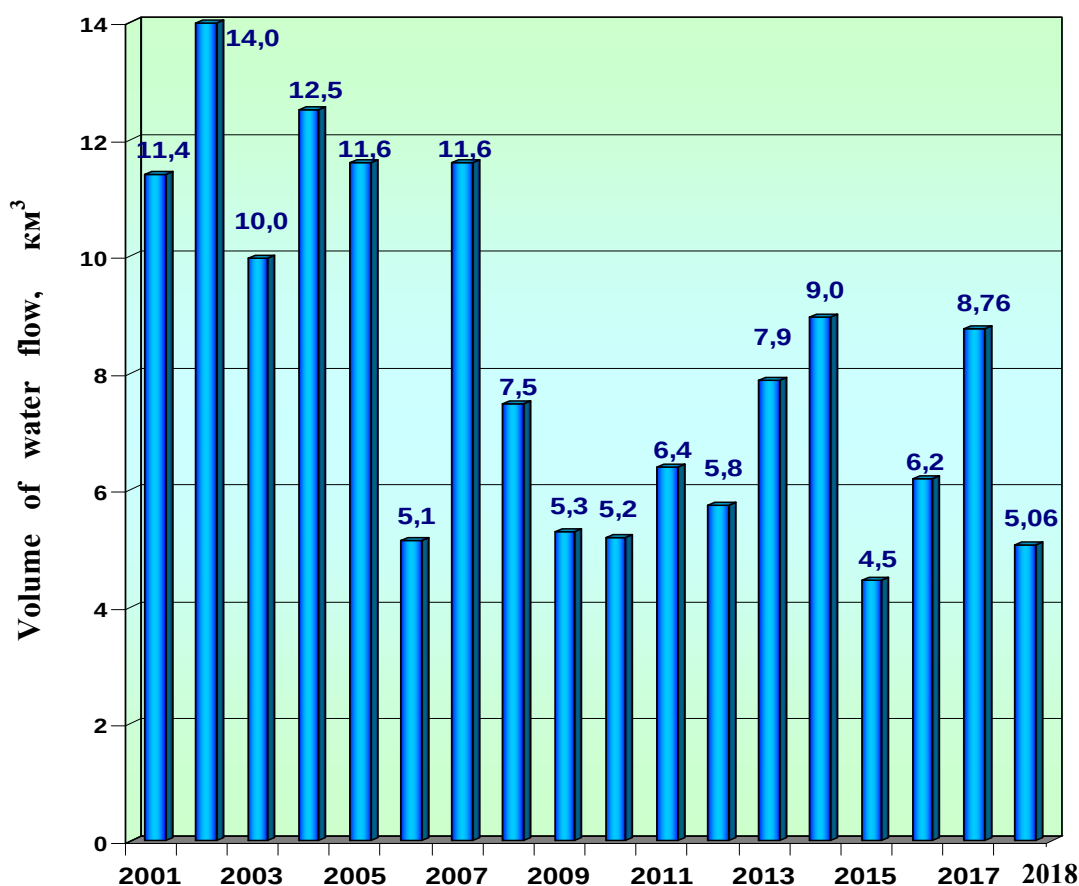
Figure 1 – Fluctuations of an annual water drain of the Ural river in the West Kazakhstan Region in 2001-2018, in km 3
